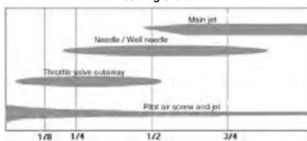
Valve throttle slide opening
